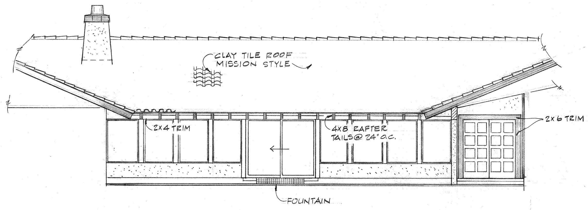
HOUSE COURT ELEVATION
