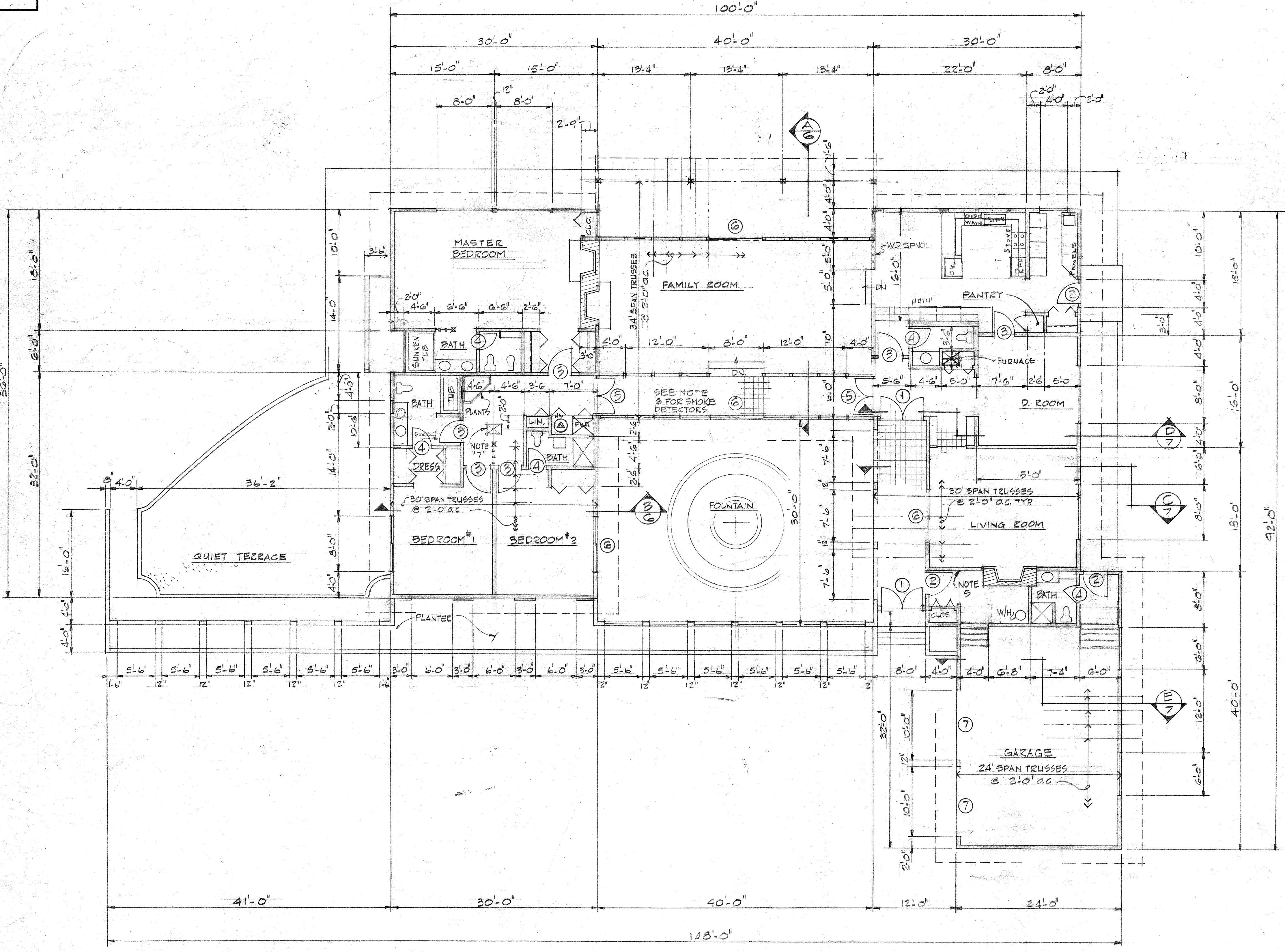
FLOOR PLAN
