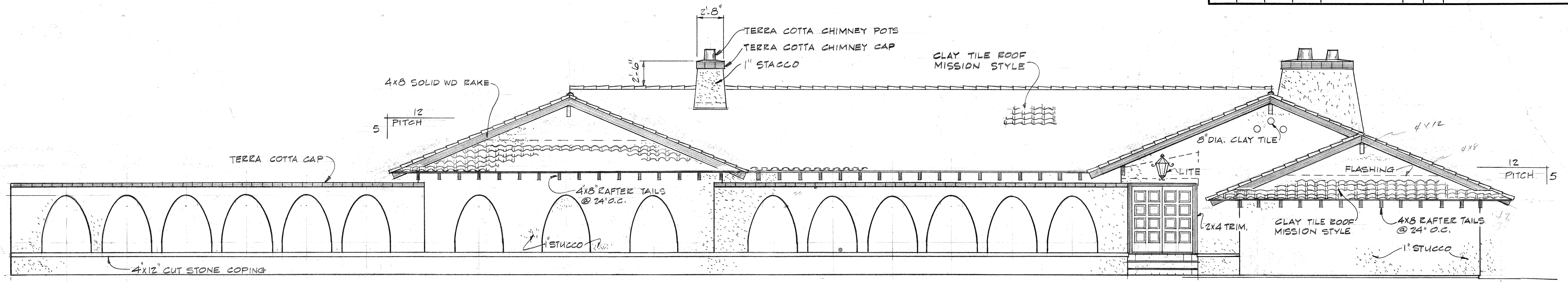
FRONT ELEVATION
