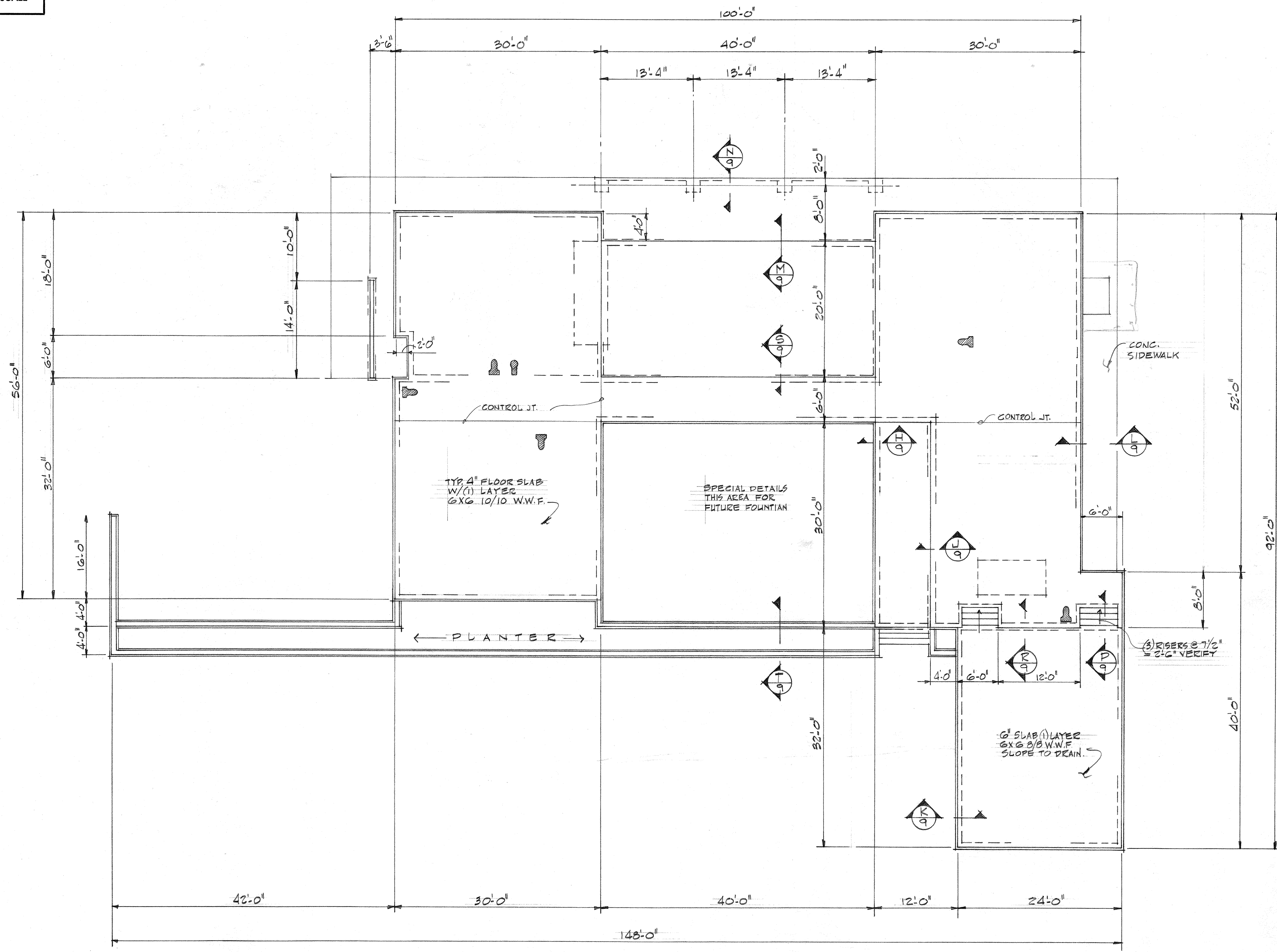
FOUNDATION PLAN
