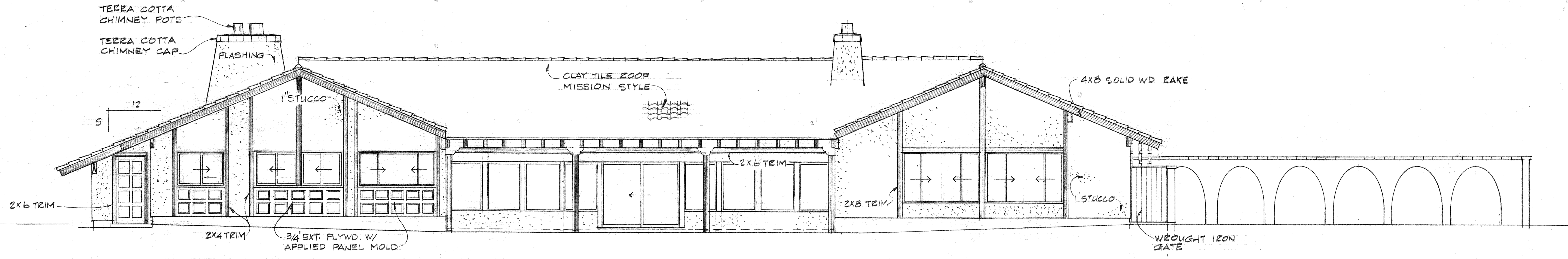
REAR ELEVATION
